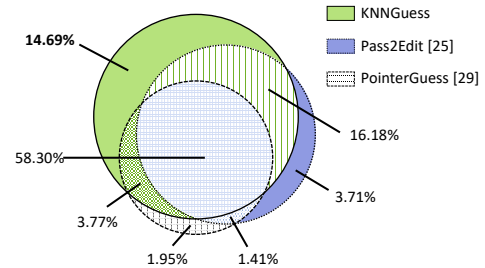
Fig. 9. The overlap ratio of passwords cracked by KNNGuess, Pass2Edit and PointerGuess. Our KNNGuess model has the highest number of cracked password pairs and the highest individual cracking ratio (i.e., 14.69%).
