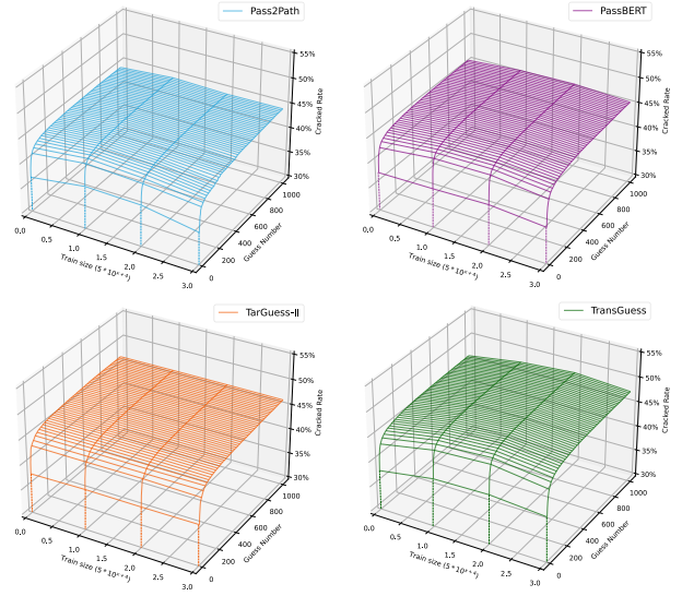
Fig. 14. The effectiveness of other models when the training set size varies in Scenario #12 (see table II). Here, we show the results of Pass2Path [13], PassBERT [26], TarGuess-II [28] and TransGuess (in this work). The x-axis represents the size of the training set, the y-axis indicates the number of guesses, and the vertical axis represents the cracking success rate of guessing. The intersections of the dashed and solid lines in the figure represent the success rates of models at the first guess.
