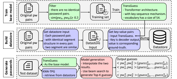
Fig. 4. The workflow of applying the KNN-TPG method to TransGuess for generating password guesses. There are three sequential steps as follows: training the base model, building the datastore, and combining KNN-TPG and TransGuess to generate password guesses. Here, n represents the number of user accounts in the test set, and the subscript A-i denotes the i -th guess in the generated password guessing list.
