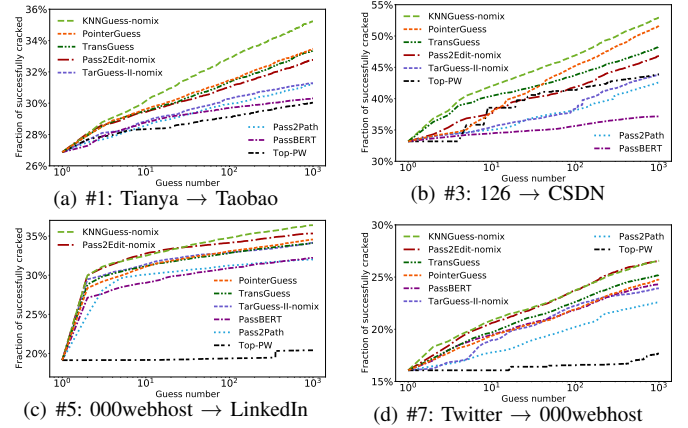
Fig. 8. Experimental results of no-mixing popular passwords in four attack scenarios. The training set is shown in Table II, and the test set is as the subtitle. Our model KNNGuess-nomix achieves the highest cracking success rate compared with other models that no-mixing popular passwords.
