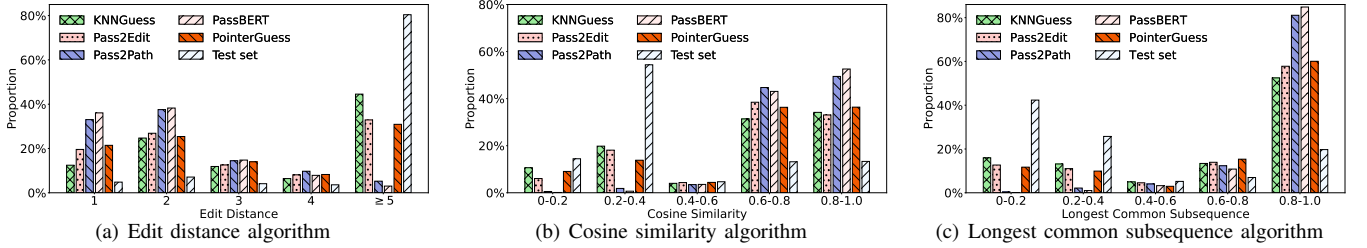
Fig. 10. The similarity distribution of password pairs cracked by 5 attack models. Figs. 10(a)-10(c) show the results using spatial distance metrics and sequence alignment-based metrics (i.e., edit distance, cosine similarity, and longest common subsequence (LCS) algorithm), to measure the similarity distribution of cracked passwords. The “Test set” represents all password pairs in the test set. KNNGuess is particularly good at predicting distant password reuse behaviors.
