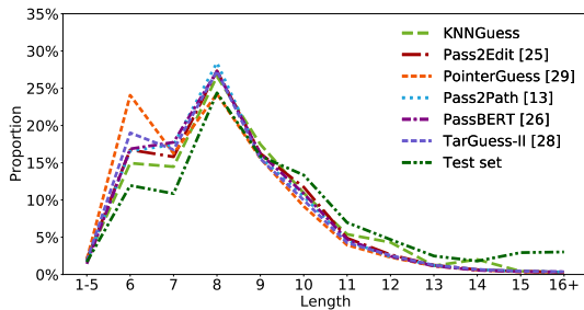
Fig. 11. The distributions of password lengths cracked by each model. Our KNNGuess best approximates the length distributions of the test set.
