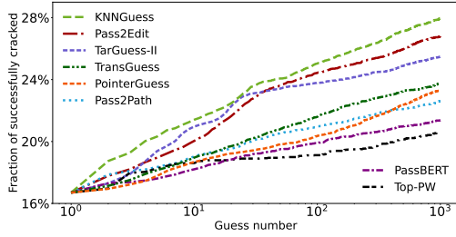
Fig. 6. The experimental results in the salted hash attack scenario #13. The training and test sets are listed in Table II. Our KNNGuess model still achieves the highest cracking success rate compare with other models.
