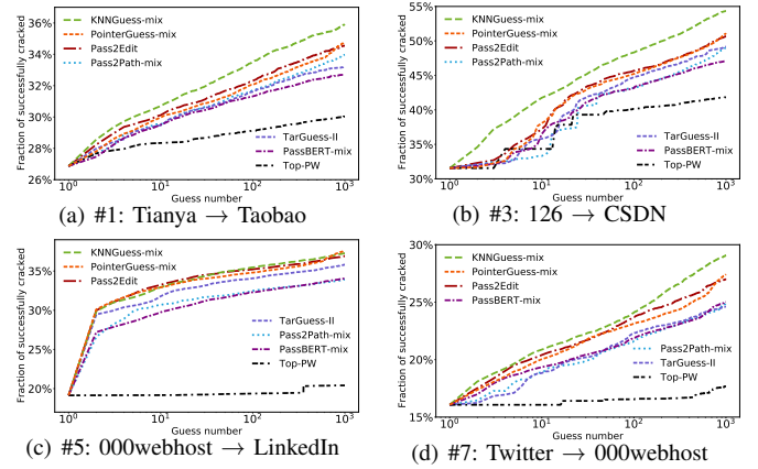
Fig. 7. Experimental results of all models mixed with popular passwords in four attack scenarios. The training set is shown in Table II, and the test set is as the subtitle. After mixing popular passwords, our KNNGuess achieves the highest cracking success rate compared with its counterparts.
