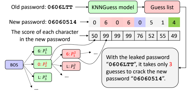
Fig. 13. Example of inputting a password pair into KNN-PSM, it provides two pieces of information: how many guesses are needed to correctly guess the new password in the event of an old password leak, and the predictability score for each character in the password, where a higher score indicates that users are more likely to choose that character.
