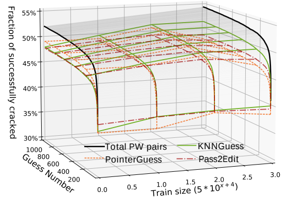
Fig. 12. KNNGuess, PointerGuess and Pass2Edit's [25] effectiveness in scenario #12 (see Table II) when the training set size changes. The x-axis represents the size of the training set, the y-axis indicates the number of guesses, and the vertical axis represents the cracking success rate of guessing. “Total PW pairs” represents the highest guess success rate achieved by combining the guess lists of the three models.
