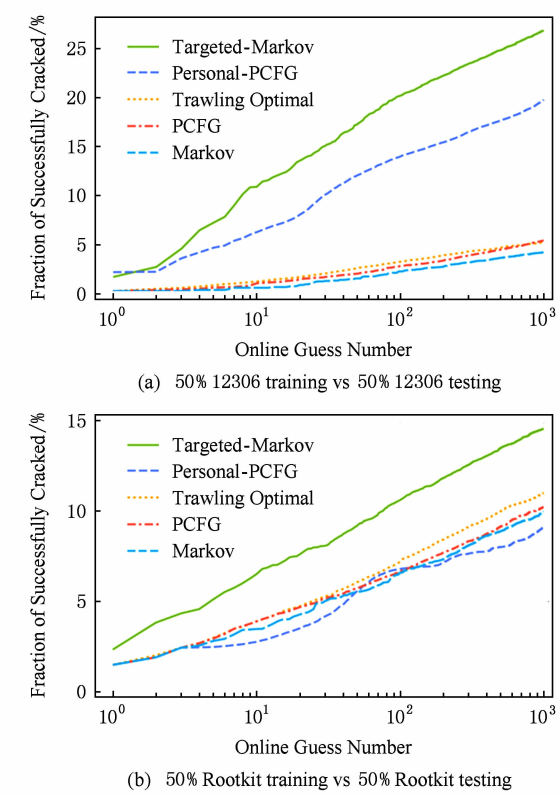
Fig. 8 Comparison of targeted guessing algorithms. 图8 定向猜测攻击算法对比
