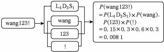
Fig. 6 Illustration of the guess generation phase of PCFG [30] .
