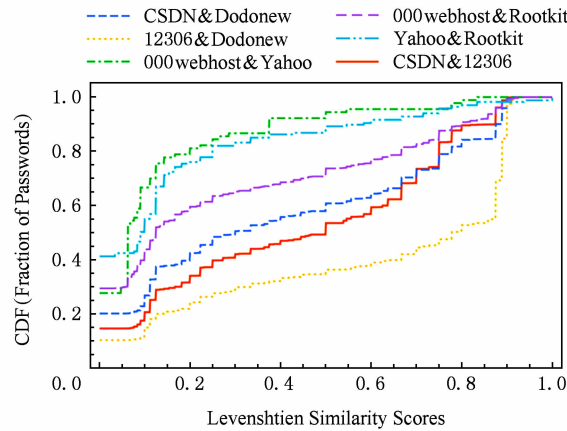
Fig. 3 Levenshtien similarity scores of indirect password reuse.
