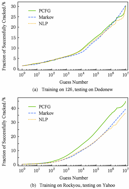
Fig. 7 Comparison of trawling guessing algorithms. 图 7 漫步猜测攻击算法对比
