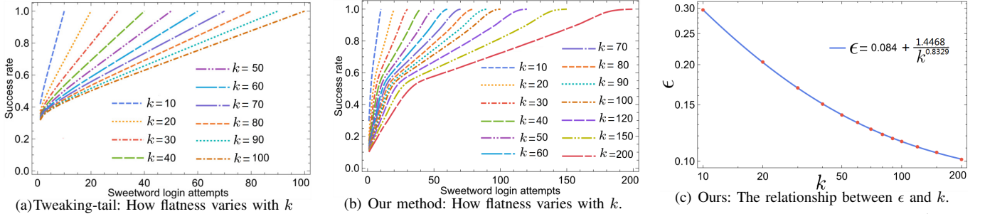
Fig. 8. How the flatness curve varies with k , trained on Dodonew-tr and tested on Dodonew-ts. Here we use tweaking-tail (under \mathcal{A}_1 ) and \frac{1}{3}\text{List} + \frac{1}{3}\text{Markov} + \frac{1}{3}\text{PCFG} (under \mathcal{A}_3 ) as examples. The sub-fig(c) shows how \epsilon ( =y|_{x=1} in sub-fig(b)) in our hybrid method evolves with k .
