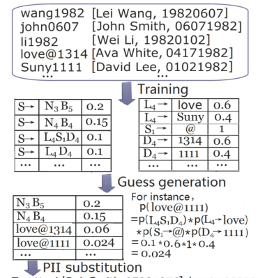
Figure 7: TarGuess-I: an illustration.
